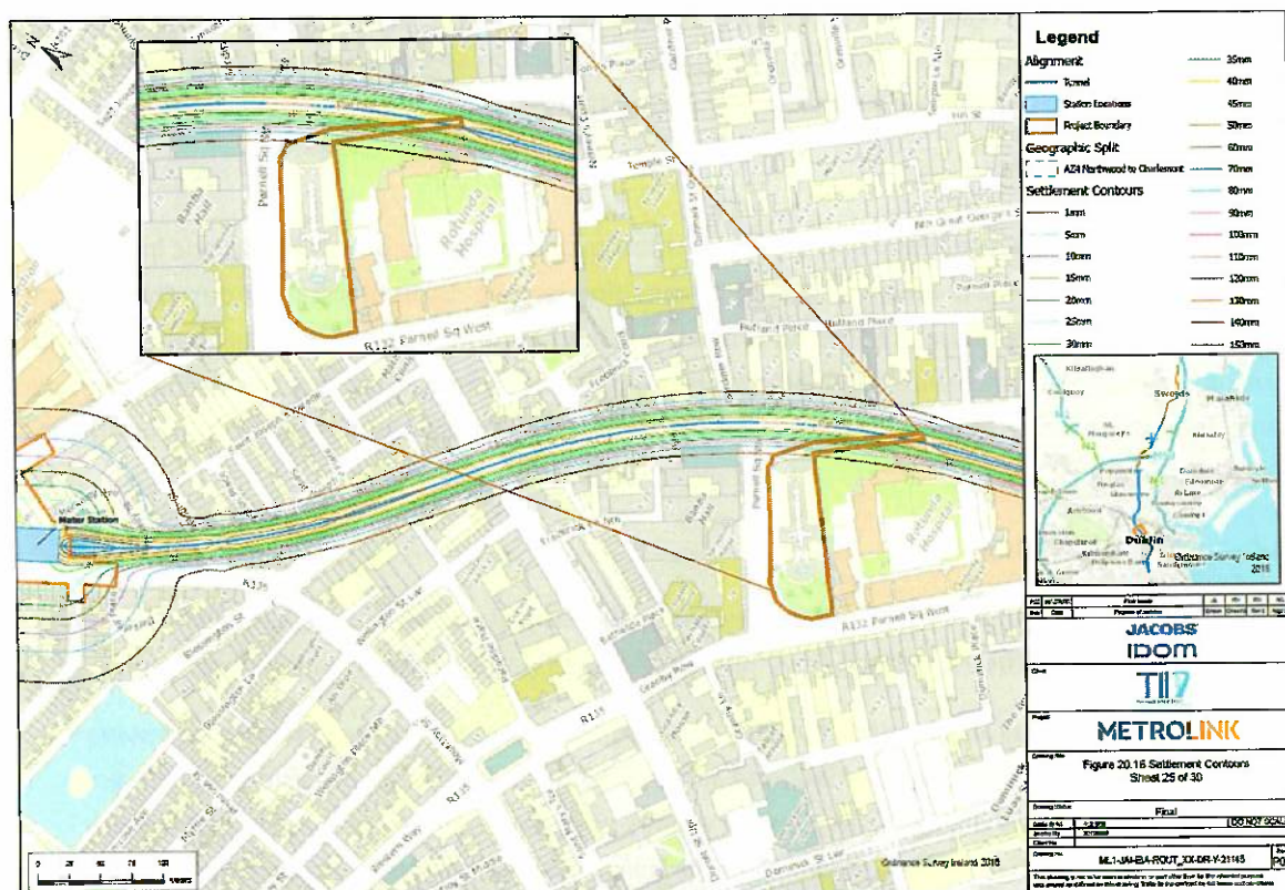
Figure 9. Settlement Contours (Extract from ML1-JAI-EIA-ROUT_XX-DR-Y-21145)
